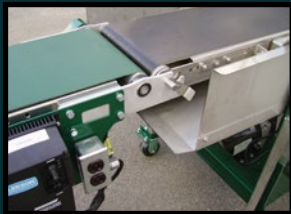
Quick-attach system
